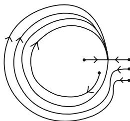
FIGURE 4.6. Attracting but not stable equilibrium.
